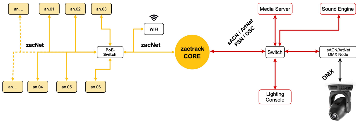
zacktrack Pro + Smart System Diagram
